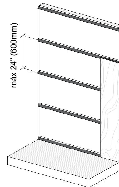
FIXING DETAIL MEASURES: INCH & MM
